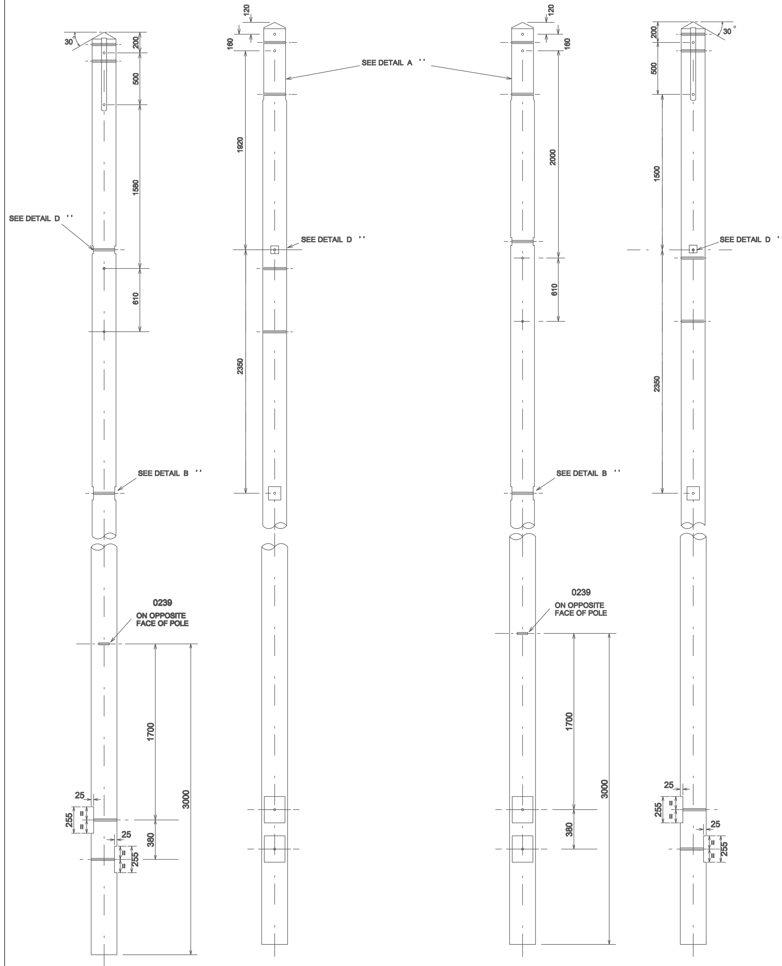
LONG LEG 0864 SHEET 1 FIG.1
