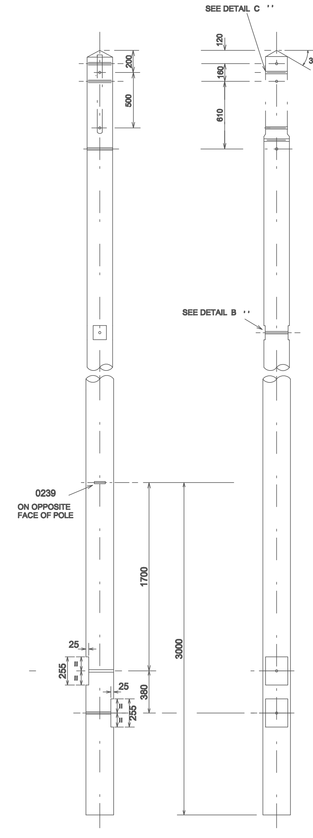
SHORT LEG 0864 SHEET 1 AND 2 FIG.3
